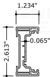
47 7075 MULLION
