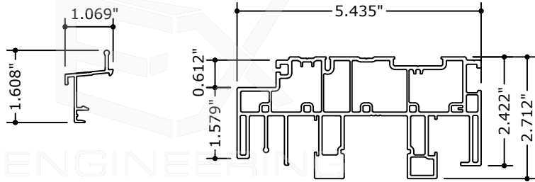
12 9991 SILL CLADDING
