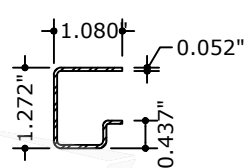
65 9598 FIXED STILE STEEL REINFORCEMENT
