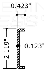
49 8760 MULLION STEEL REINFORCEMENT
