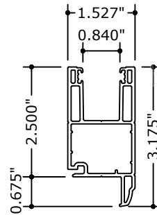
37 7508-M MOBILE HORIZONTAL RAIL
