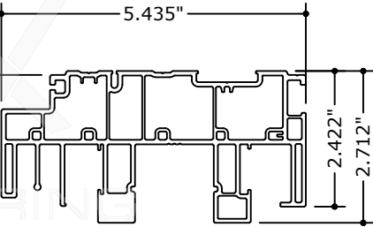
15 7002 HEAD PROFILE
